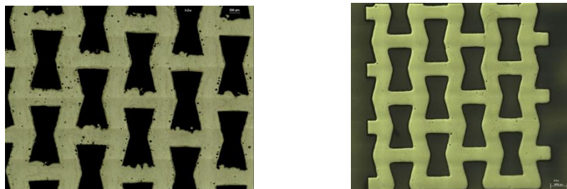
Figure 1: Shape defects and porosity distribution as a function of printing parameters, exposure time, laser power, and printing direction, etc.
